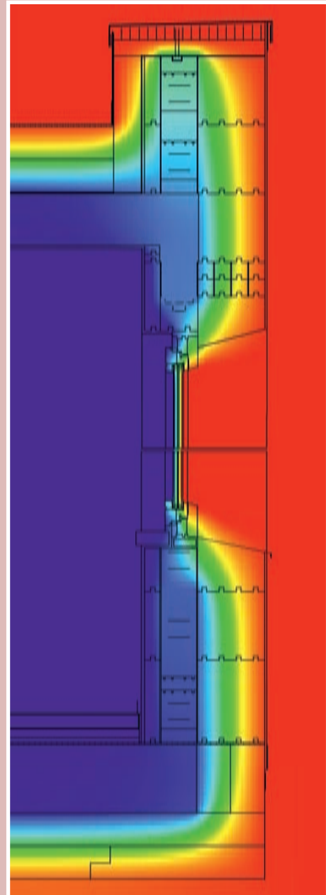
Isotherm profile of an external wall with insulating concrete forms (ICF), base plate foundation, and flat roof
